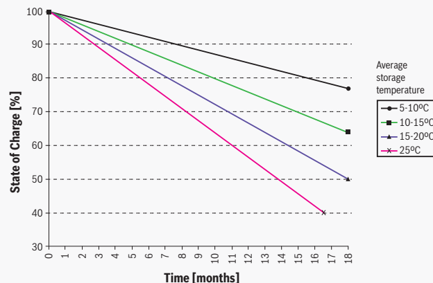
Example of self discharge on a lead acid battery
